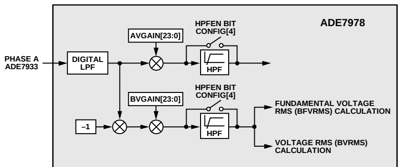
Figure 70. Phase B Voltage Calculation in 3P4W Delta Configuration (CONSEL = 11 in the ACCMODE Register)
