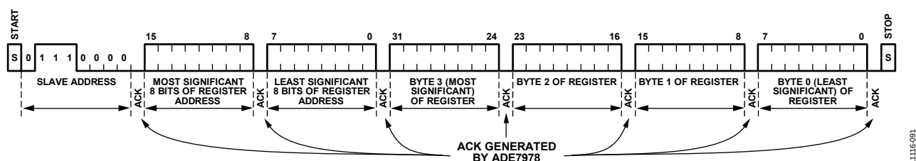
Figure 116. I 2 C Write Operation of a 32-Bit Register
