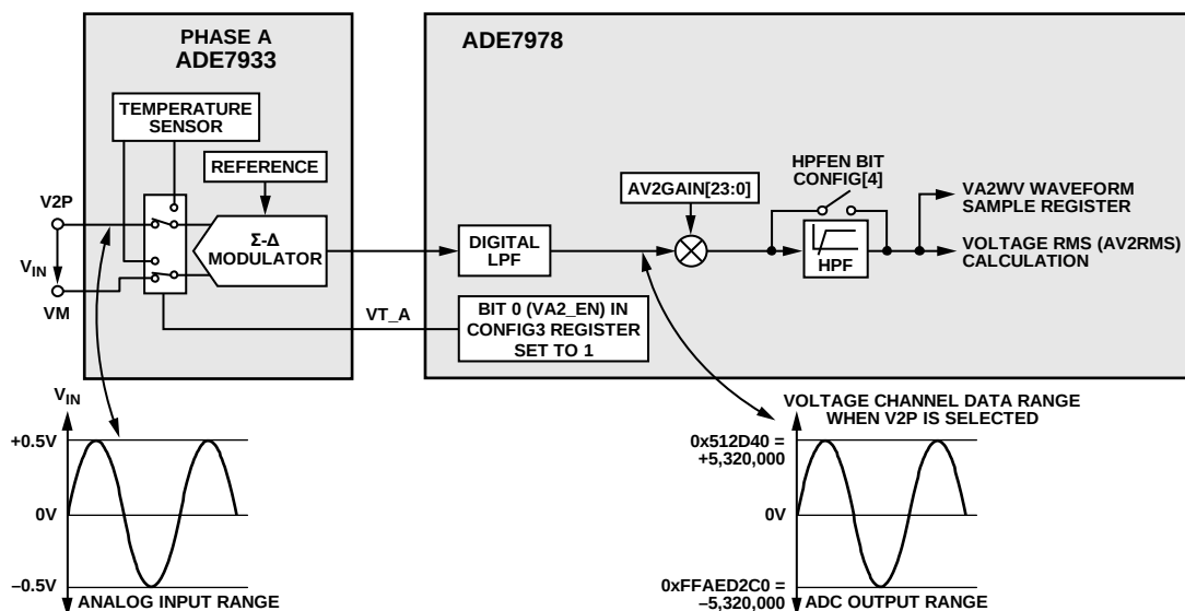
Figure 48. Phase A V2P Channel Datapath (ADE7933 Only)
