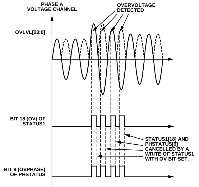
Figure 64. Overvoltage Detection
