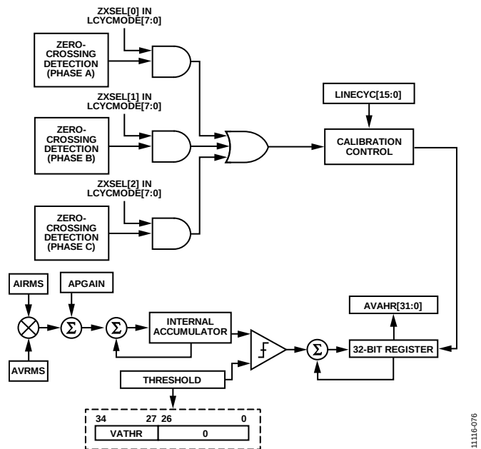
Figure 82. Line Cycle Apparent Energy Accumulation Mode
