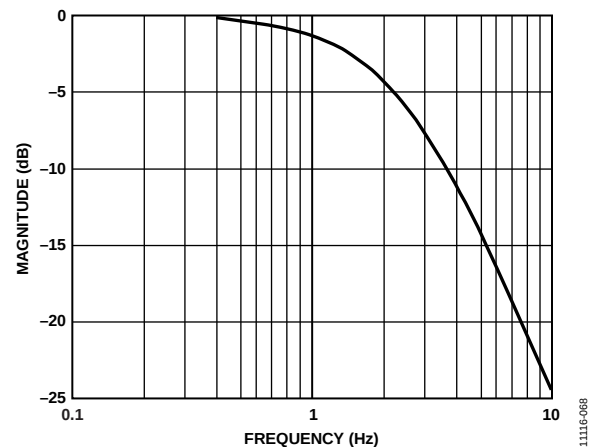
Figure 73. Frequency Response of the LPF Used to Filter Instantaneous Power in Each Phase: LPSSEL Bit of CONFIG Register Set to 0 (Default)
