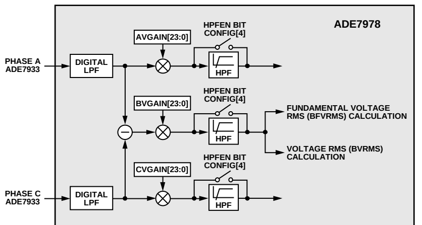
Figure 69. Phase B Voltage Calculation in 3P3W Delta Configuration (CONSEL = 01 in the ACCMODE Register)
