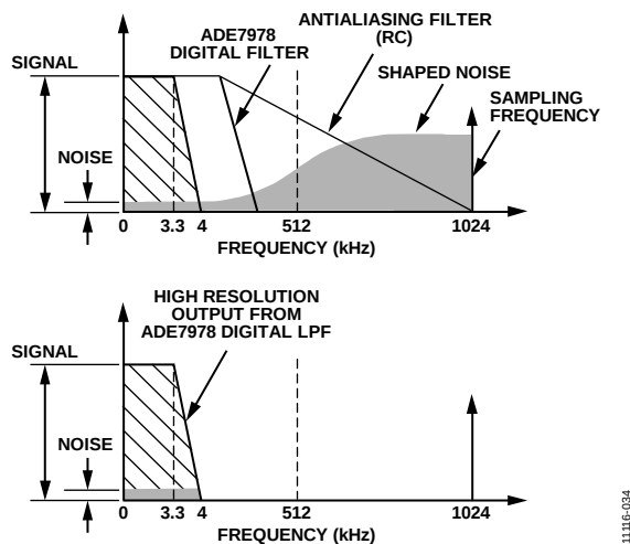
Figure 40. Noise Reduction Due to Oversampling and Noise Shaping in the Analog Modulator
