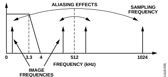
Figure 41. Aliasing Effects
