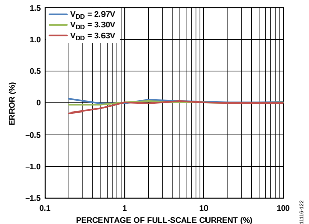
Figure 17. Apparent Energy Error as a Percentage of Reading over Power Supply, PF = 1, T_A = 25^\circ\text{C}
