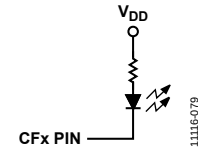
Figure 85. CFx Pin Recommended Connection
