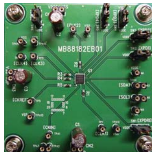
Evaluation Board (MB88182EB01)
