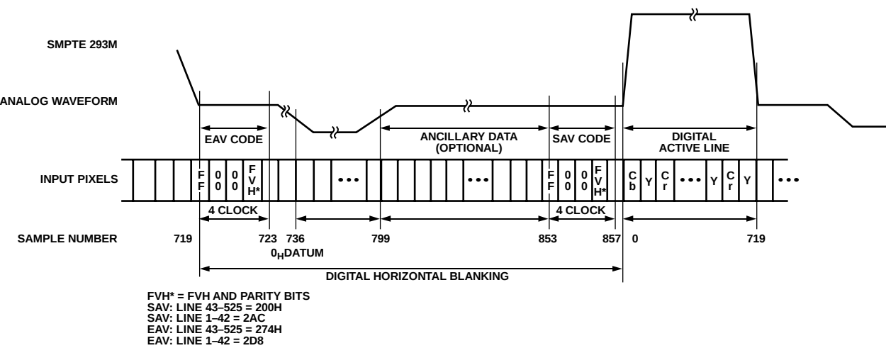
Figure 134. EAV/SAV Input Data Timing Diagram (SMPTE 293M)
