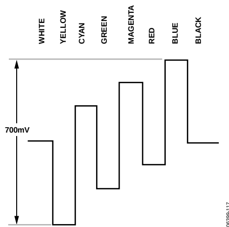
Figure 115. Pb Levels—NTSC
