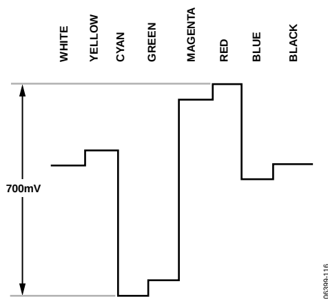
Figure 114. Pr Levels—NTSC
