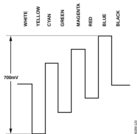
Figure 118. Pb Levels—PAL
