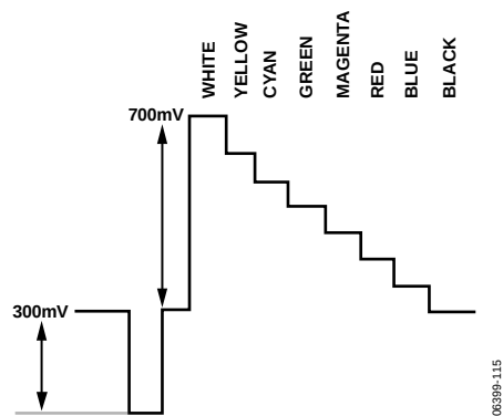
Figure 113. Y Levels—NTSC
