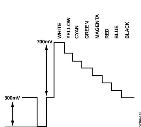
Figure 116. Y Levels—PAL
