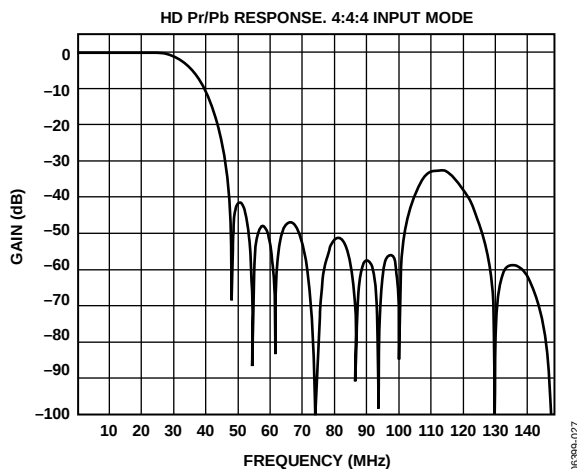
Figure 26. HD 4× Oversampling, PrPb (SSAF) Filter Response (4:4:4 Input)
