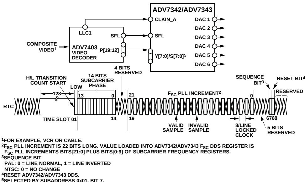
Figure 59. SD Subcarrier Frequency Lock Timing and Connections Diagram (Subaddress 0x84, Bits [2:1] = 11)
