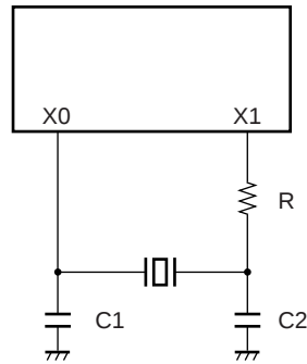
Example oscillation circuit
