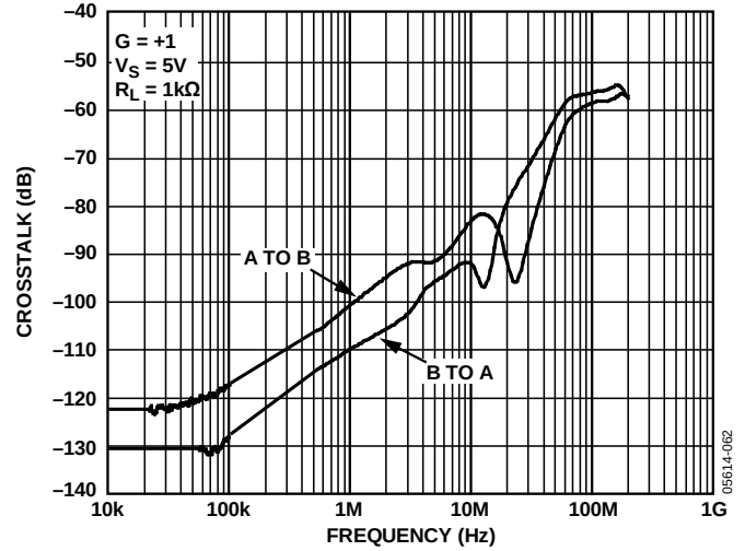
Figure 38. Crosstalk Output to Output
