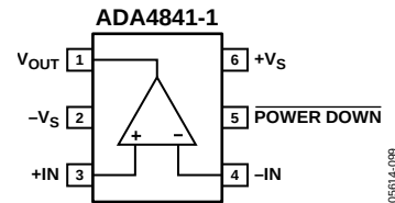
Figure 2. 6-Lead SOT-23 (RJ)
