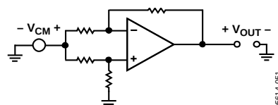
Figure 44. Common-Range Subtractor
