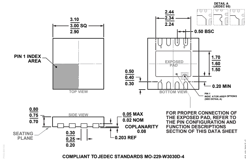
COMPLIANT TO JEDEC STANDARDS MO-229-W3030D-4 Figure 55. 8-Lead Lead Frame Chip Scale Package [LFCSP] 3 mm x 3 mm Body and 0.75 mm Package Height (CP-8-11) Dimensions shown in millimeters
