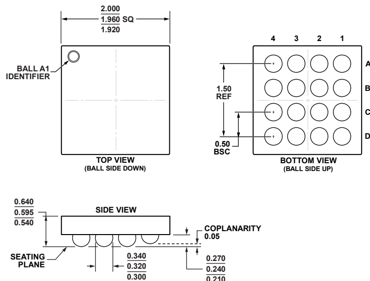
Figure 52. 16-Ball Wafer Level Chip Scale Package [WLCSP] (CB-16-3) Dimensions shown in millimeters
