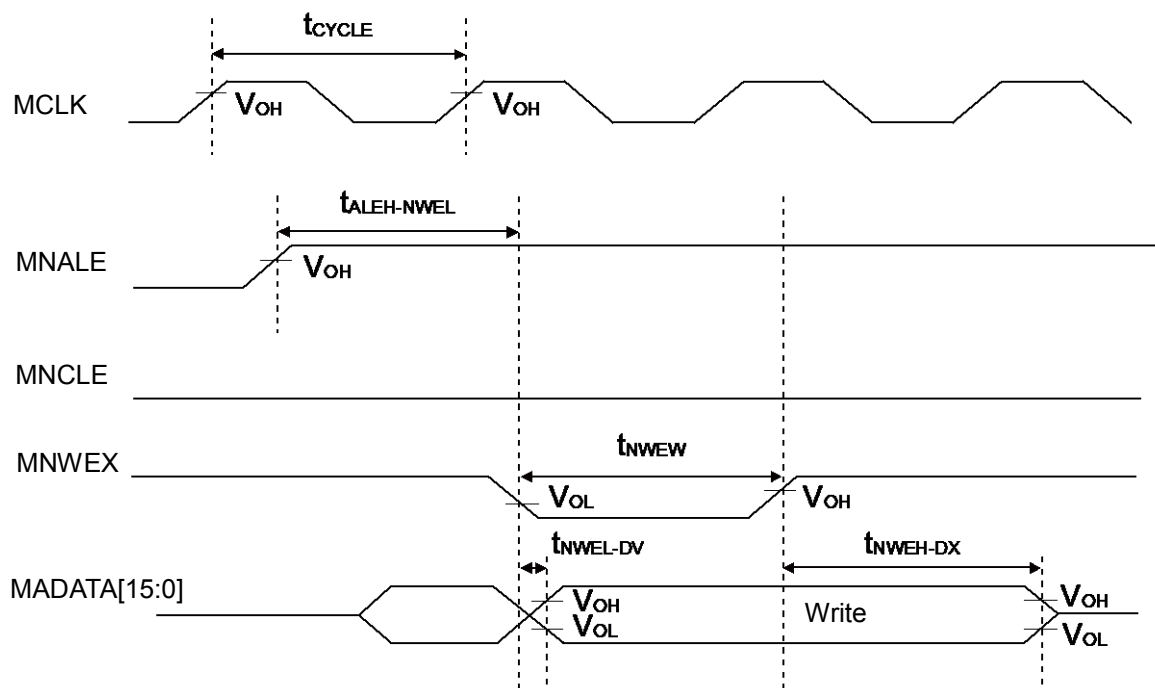
NAND Flash Address Write
