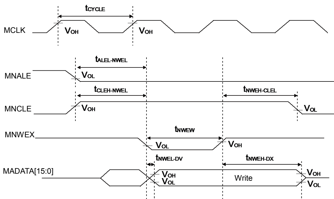
NAND Flash Command Write
