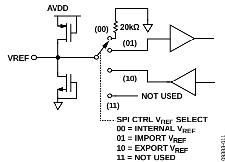
Figure 39. Equivalent V_{REF} Input/Output Circuit
