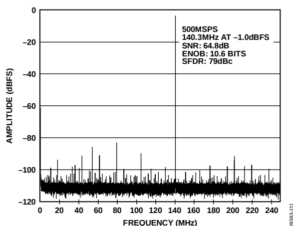
Figure 11. AD9434-500 64k Point Single-Tone FFT; 500 MSPS, 140.3 MHz
