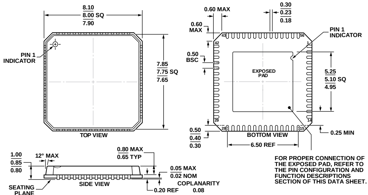
COMPLIANT TO JEDEC STANDARDS MO-220-VLLD-2 Figure 53. 56-Lead Lead Frame Chip Scale Package [LFCSP_VQ] 8 mm x 8 mm Body, Very Thin Quad (CP-56-5) Dimensions shown in millimeters
