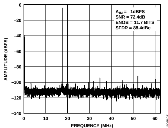
Figure 35. Single-Tone 16k FFT with f_{IN} = 140 MHz at f_{SAMPLE} = 122.88 MSPS
