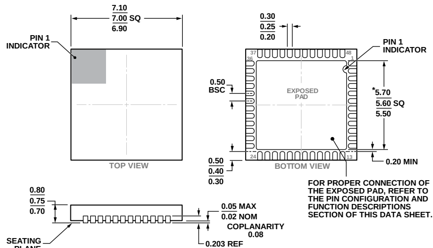
Figure 77. 48-Lead Lead Frame Chip Scale Package [LF CSP_WQ] 7 mm x 7 mm Body, Very Very Thin Quad (CP-48-13) Dimensions shown in millimeters
