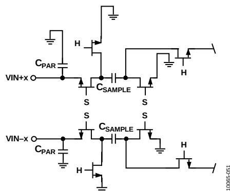
Figure 55. Switched-Capacitor Input Circuit
