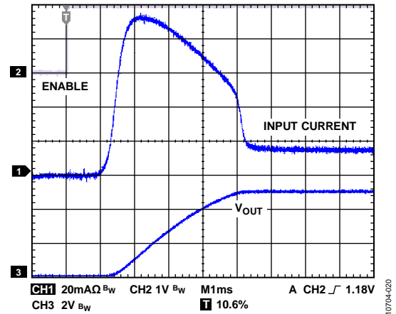
Figure 19. Typical Turn-On Time and Inrush Current, V_{IN} = 5V , C_{OUT} = 47\mu F , 330\Omega Load
