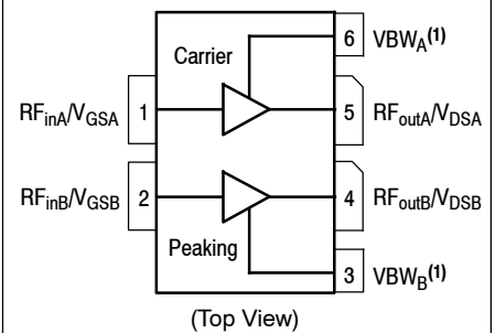
Figure 1. Pin Connections
