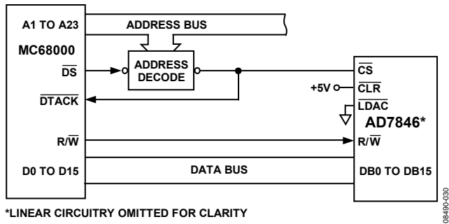
Figure 28. AD7846-to-MC68000 Interface
