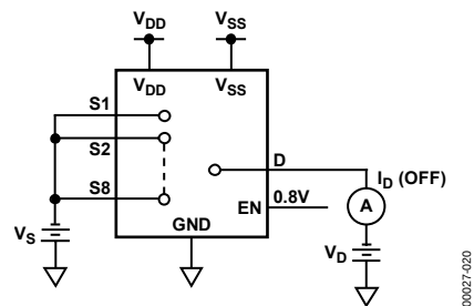
Figure 20. I_D (OFF)
