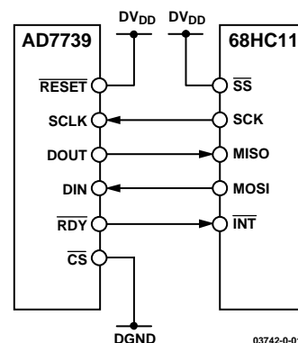
Figure 12. AD7739 to Host Device Interface, SPI
