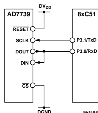
Figure 14. AD7739 to Host Device Interface, 2-Wire Configuration
