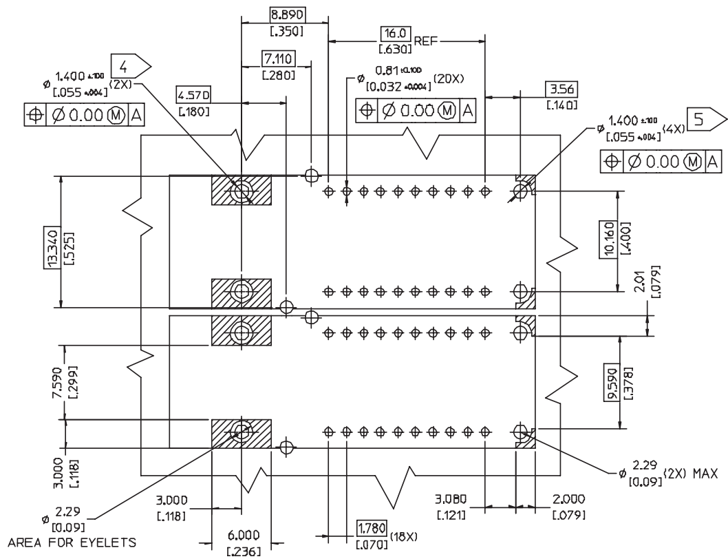
Figure 8. Board Layout
