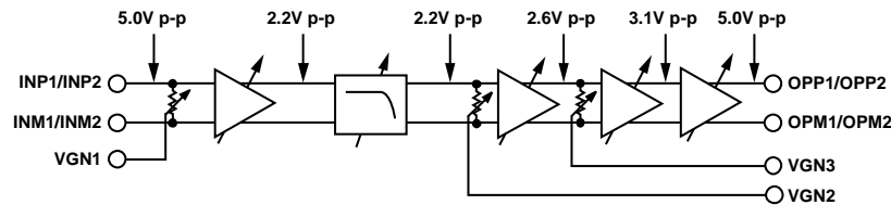
Figure 86. Maximum Signal Levels; Single Channel Shown
