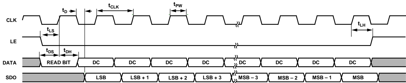
Figure 3. Read Mode Timing Diagram
