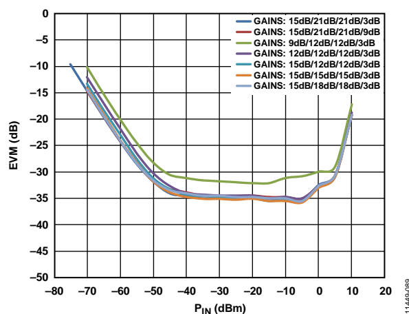
Figure 83. EVM vs. Input Power over Gain Code; Filter Mode = 63 MHz, QPSK, 50 MSPS, 1.5 V p-p Differential Output Level Maintained
