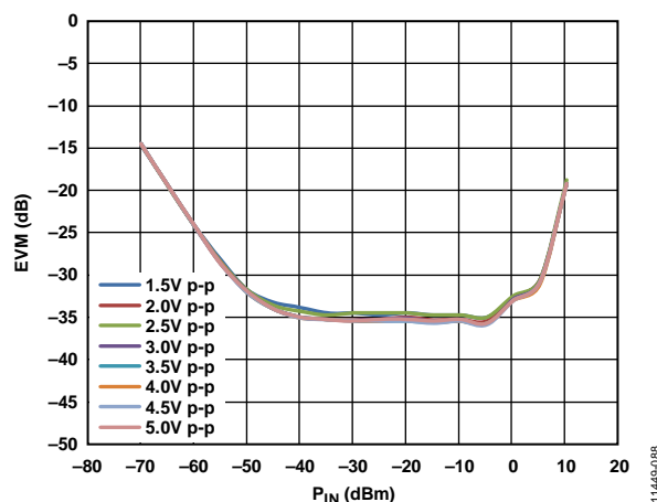
Figure 82. EVM vs. Input Power over Output Level; Filter Corner = 63 MHz, QPSK, 50 MSPS, Gain Code = 0000000
