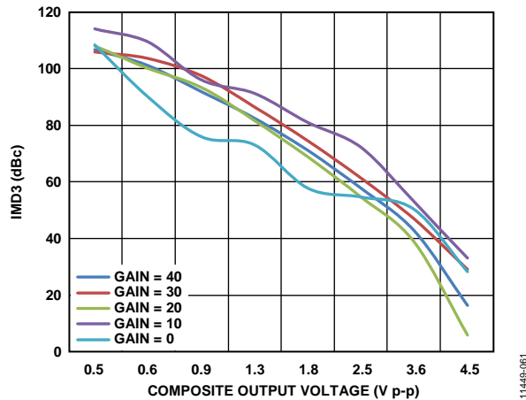
Figure 60. IMD3 vs. Composite Output Voltage over VCM; VGN1/VGN2/VGN3 = 1 V, 125 MHz and 126 MHz Tones
