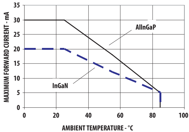
Figure 7. Maximum forward current vs. ambient temperature For AlInGaP & InGaP Derating based on T_{JMAX} = 95^{\circ}
