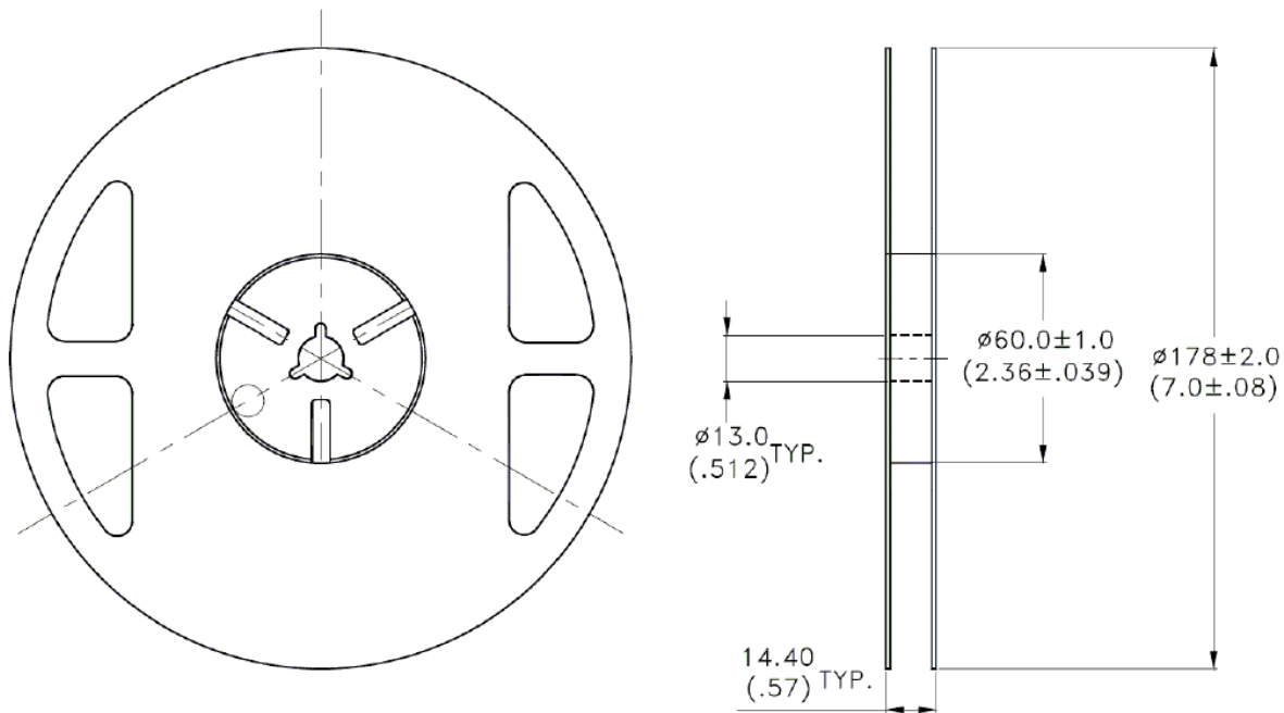
Figure 12. Reel dimensions [1]
