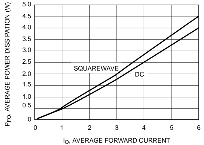
Figure 7. Power Dissipation
