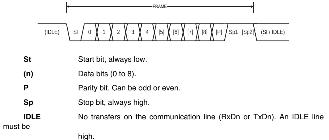
Figure 17-4. Frame Formats
