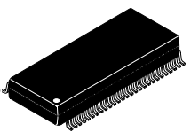
DWB SUFFIX CASE 1390 54-LEAD SOICW-EP
