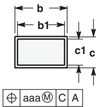
SECTION W-W
