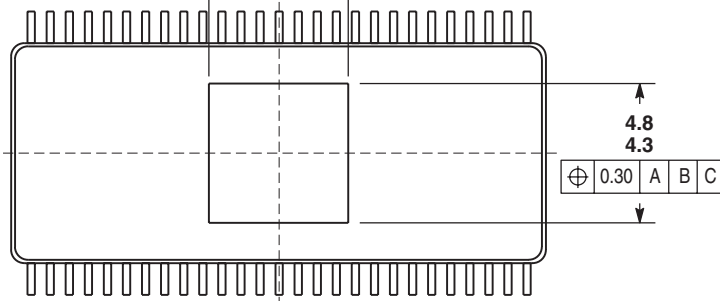
VIEW C-C
