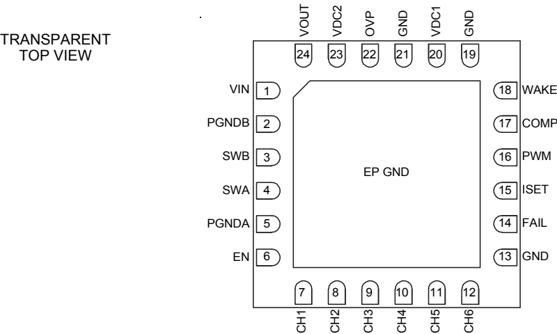
Figure 3. 34845 Pin Connections
