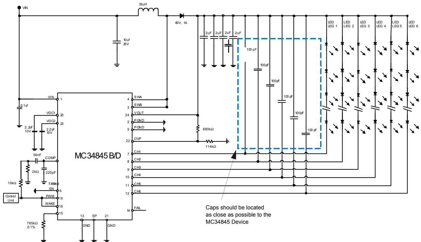
Figure 11. Typical Application Circuit for Single Wire Control, f_s = 300 \text{ kHz} ( V_{IN} = 8.0\text{V} , I_{LED} = 20 \text{ mA/channel} , 14 LEDs/channel, OVP = 49V, V_{PWM} = 3.3\text{V} )
