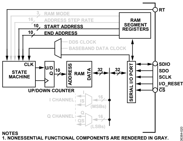
Figure 40. RAM Load/Retrieve Operation
