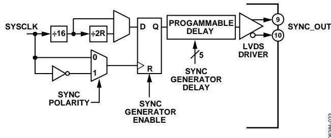
Figure 56. Sync Generator
