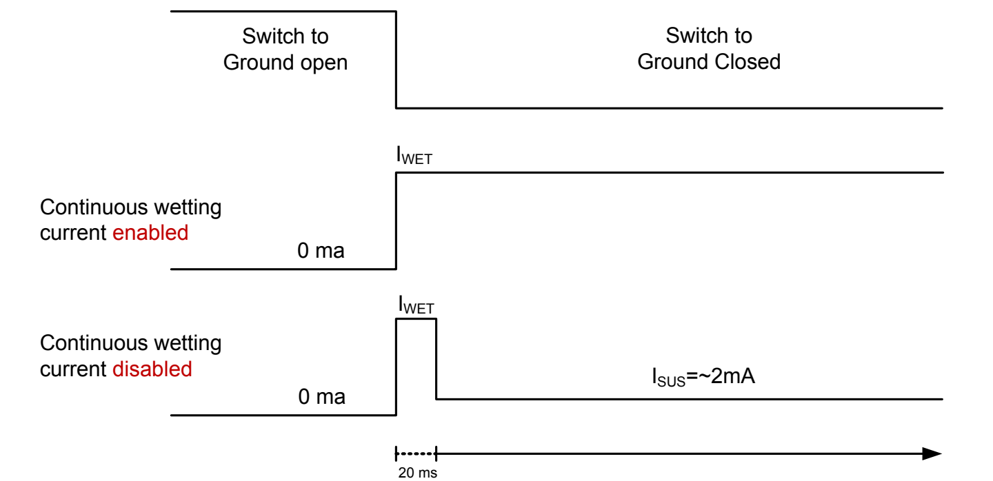
Figure 22. Pulsed/Continuous Wetting Current Configuration
