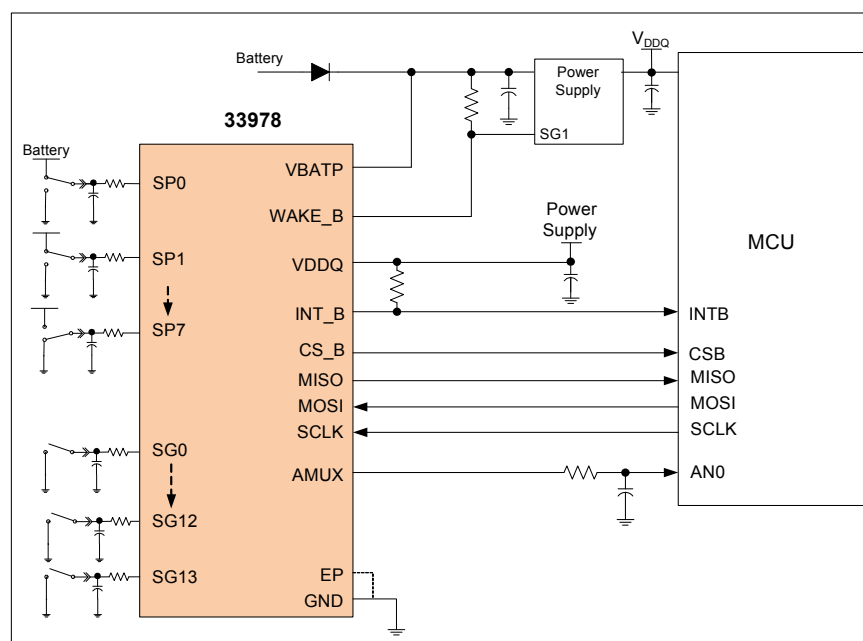
Figure 1. 33978 Simplified Application Diagram
