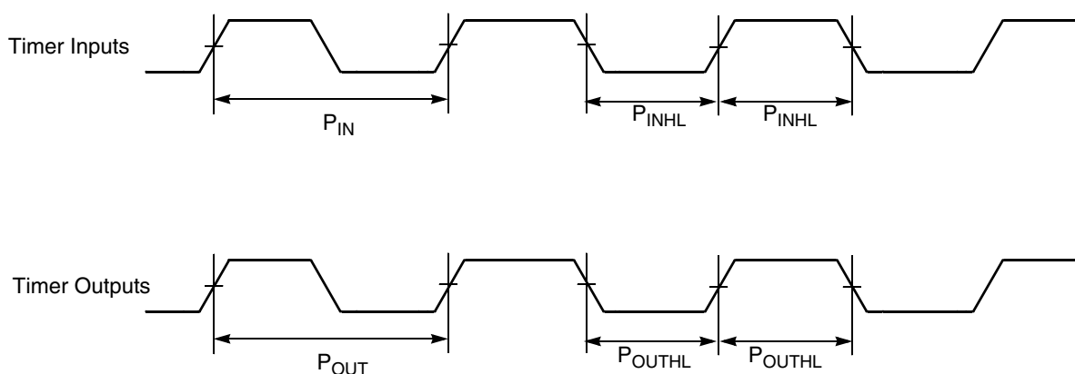
Figure 36. Timer Timing
