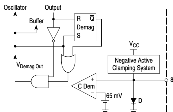
Figure 39. Demagnetization Block
