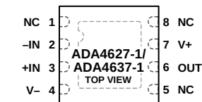
Figure 2. 8-Lead SOIC_N (R-8)
