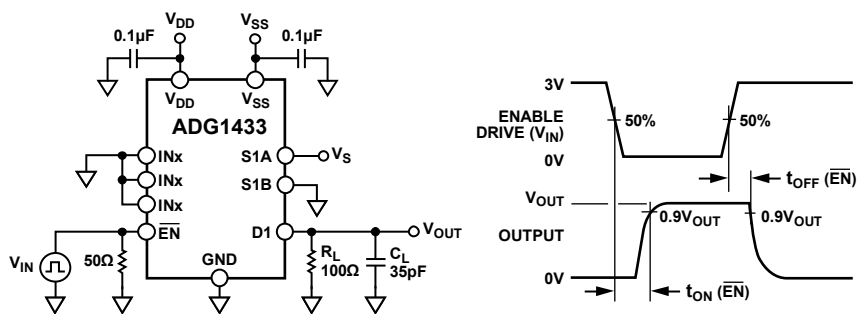
Figure 30. Enable Delay, t_{ON}(\overline{EN}) , t_{OFF}(\overline{EN})
