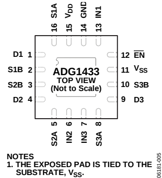
Figure 5. ADG1433 LFCSP Pin Configuration
