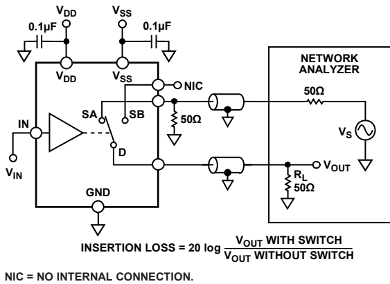
Figure 33. Bandwidth
