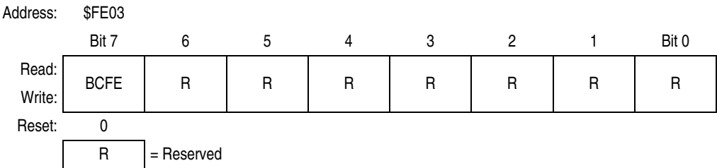
Figure 20-22. Break Flag Control Register (BFCR)
