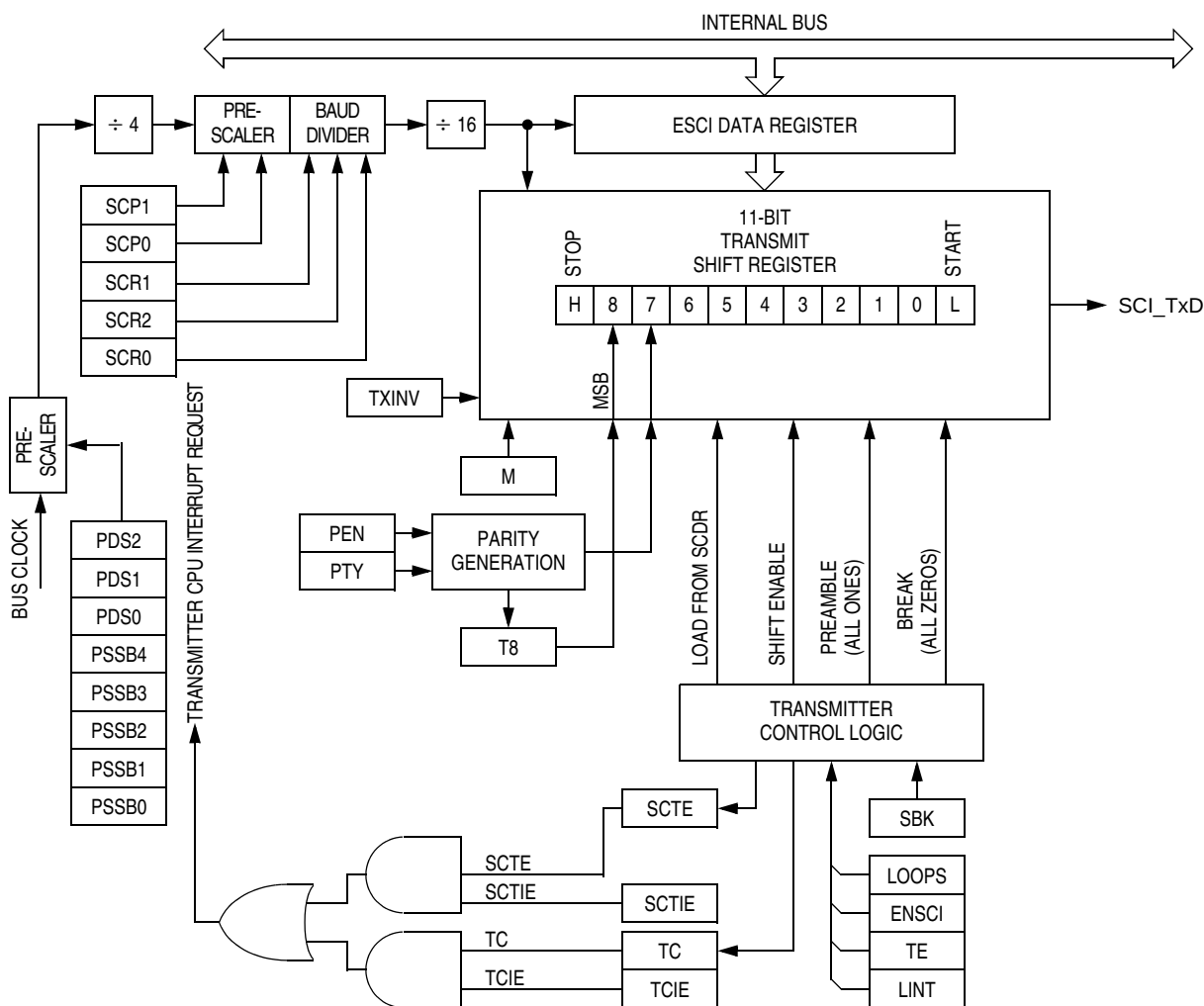
Figure 19-4. ESCI Transmitter
