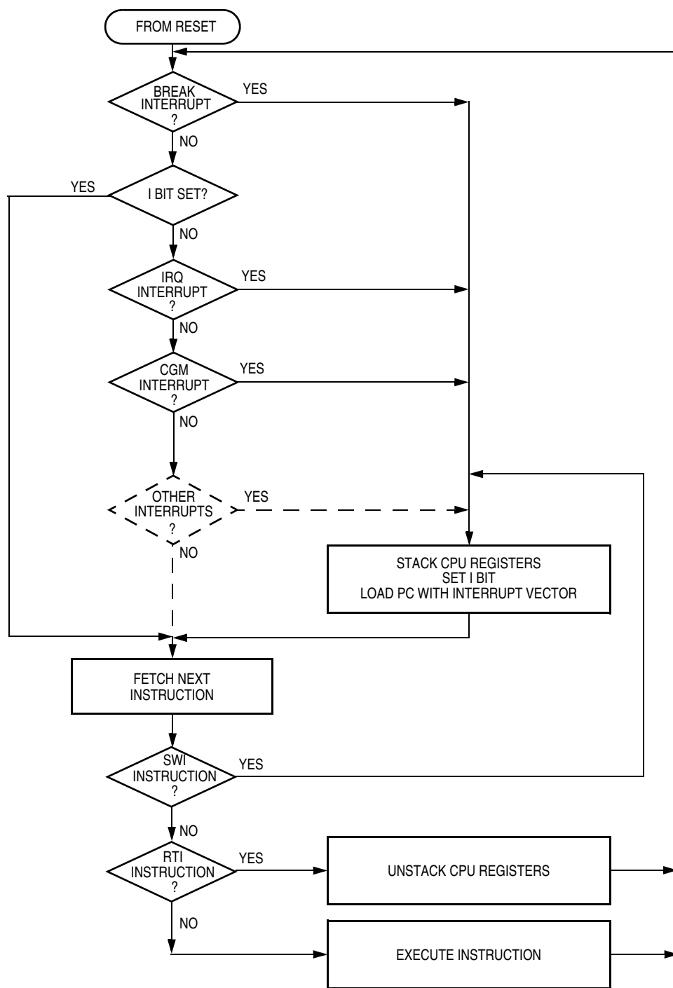
Figure 4-5. Interrupt Processing
