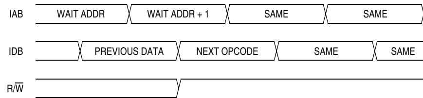
Figure 20-15. Wait Mode Entry Timing
