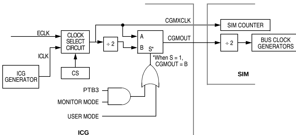
Figure 10-3. ICG Clock Signals
