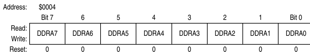
Figure 9-3. Data Direction Register A (DDRA)
