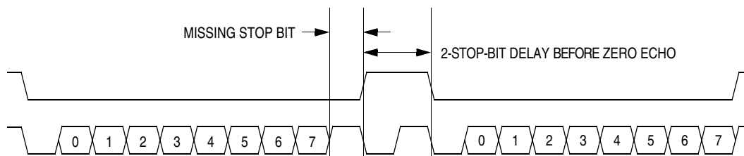
Figure 13-9. Break Transaction
