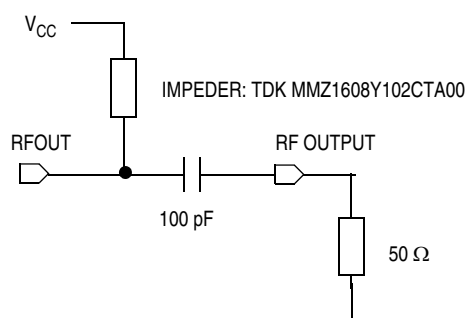
Figure 14-4. Output Power Measurement Configurations
