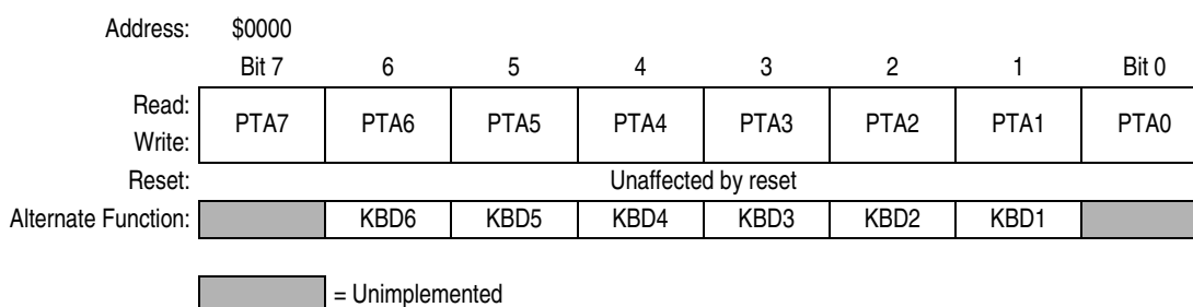
Figure 9-2. Port A Data Register (PTA)
