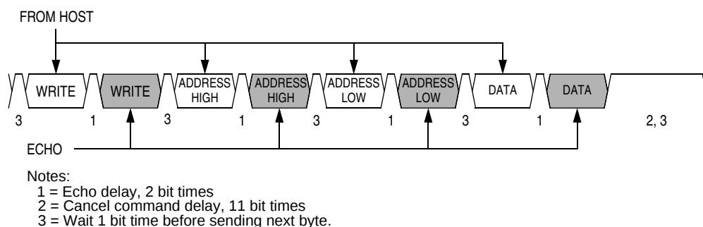
Figure 13-11. Write Transaction
