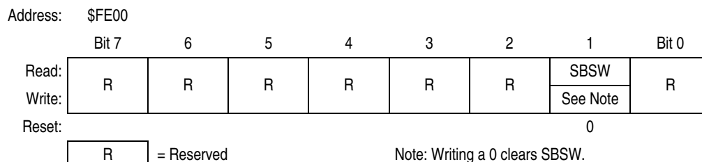
Figure 10-17. SIM Break Status Register (SBSR)
