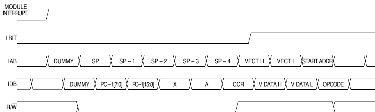
Figure 10-8. Interrupt Entry
