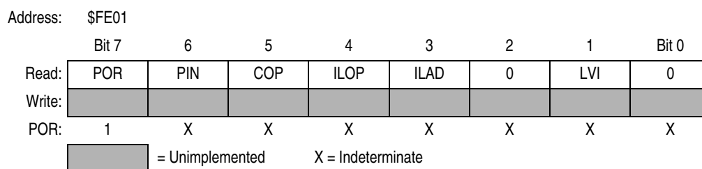
Figure 10-18. SIM Reset Status Register (SRSR)
