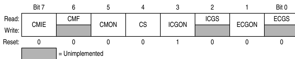
Figure 6-11. ICG Control Register (ICGCR)
