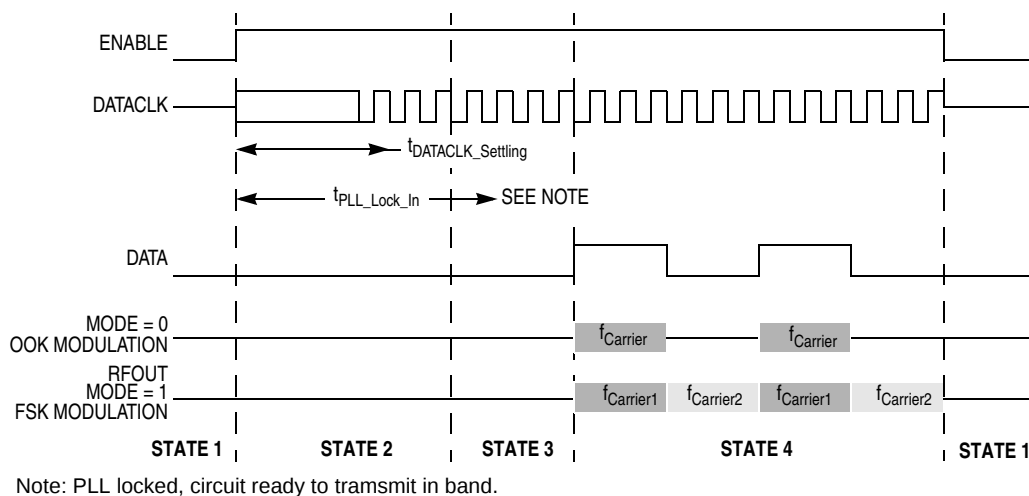
Figure 12-4. Signals, Waveforms, and Timing Definitions
