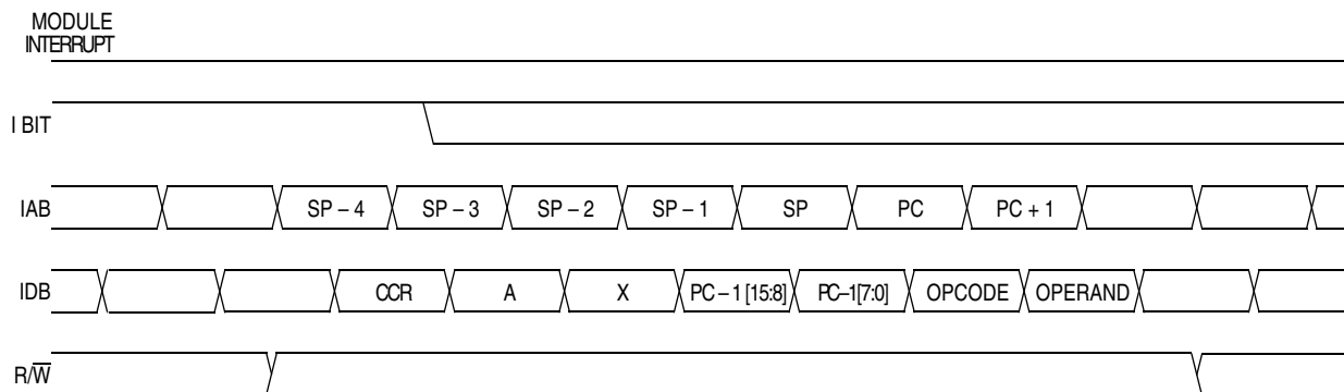
Figure 10-9. Interrupt Recovery
