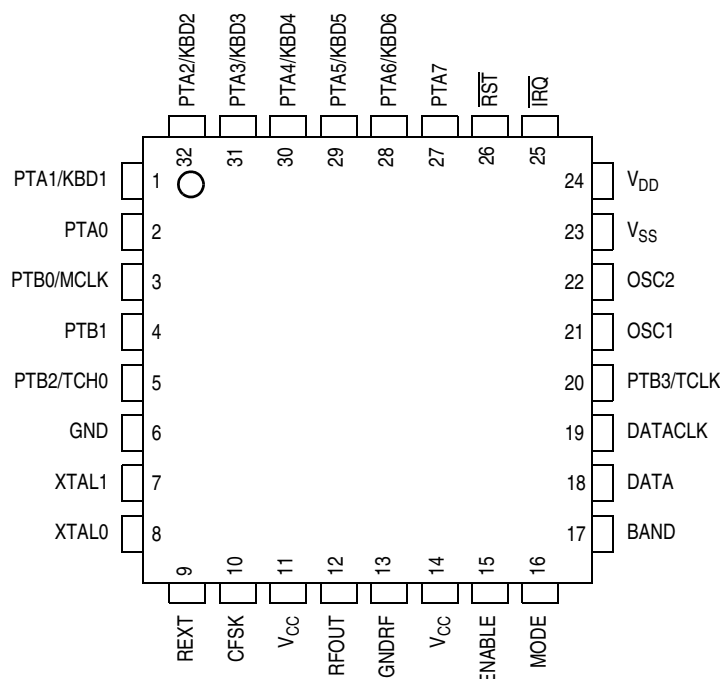
Figure 1-2. LQFP Pin Assignments
