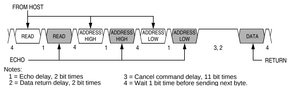
Figure 13-10. Read Transaction
