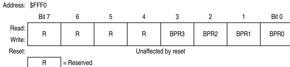
Figure 2-5. FLASH 2TS Block Protect Register (FLBPR)
