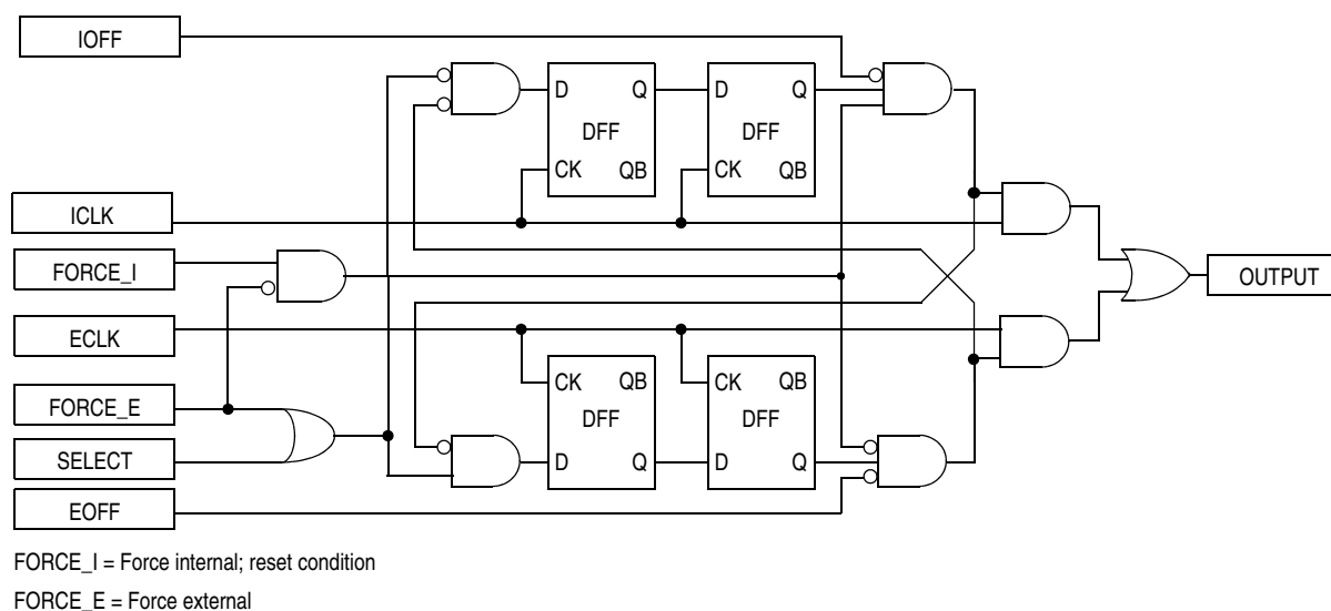
Figure 6-6. Synchronizing Clock Switcher Circuit Diagram
