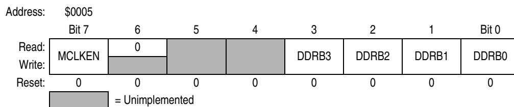
Figure 9-6. Data Direction Register B (DDRB)
