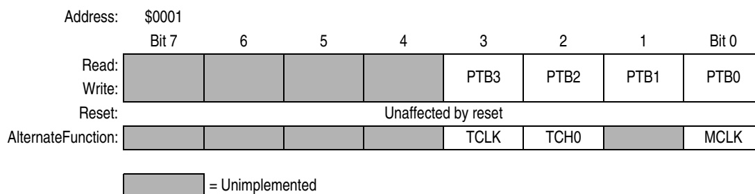
Figure 9-5. Port B Data Register (PTB)
