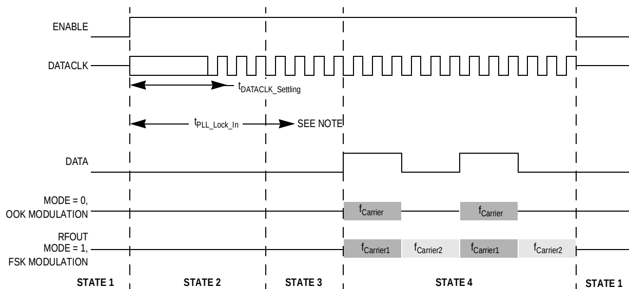
Figure 16-3. Signals, Waveforms, and Timing Definitions
