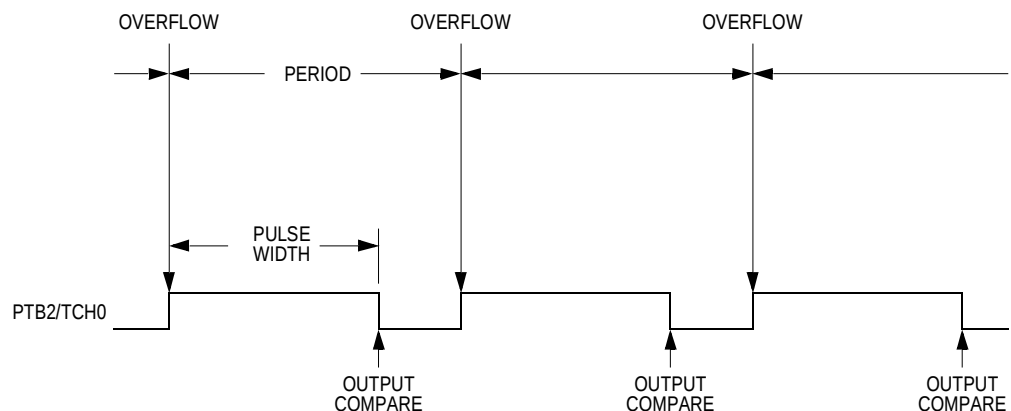
Figure 15-3. PWM Period and Pulse Width
