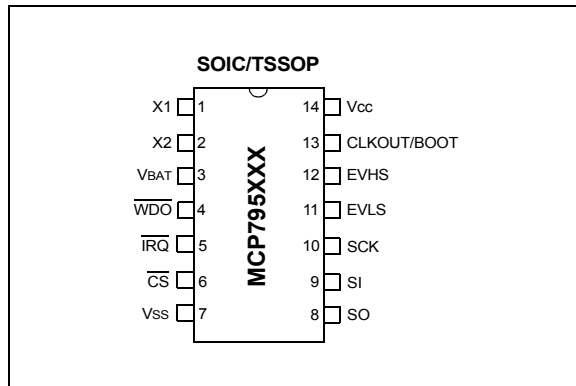
FIGURE 2-1: DEVICE PINOUTS
