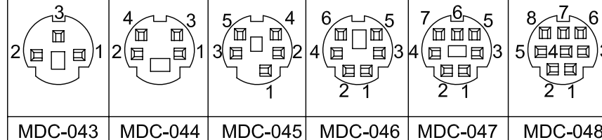
MATING VIEW
