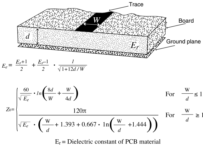
Figure 37: Microstrip Formulas
