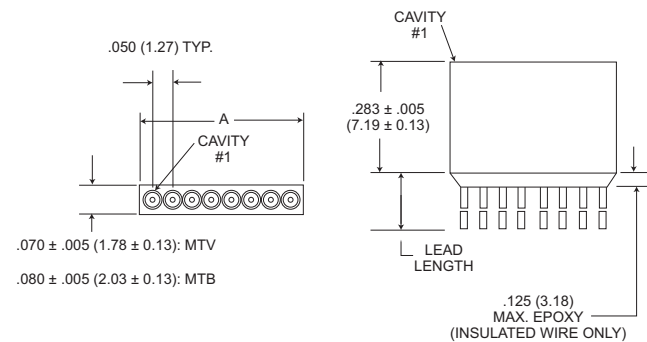
Plug
