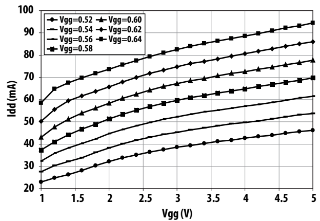
Figure 16. I-V curve
