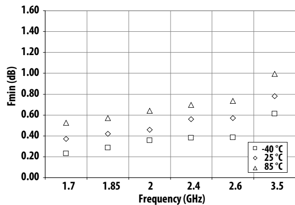
Figure 18. F_{min} vs Frequency and Temperature tuned for Optimum OIP3 and F_{min} at 5V 50mA
