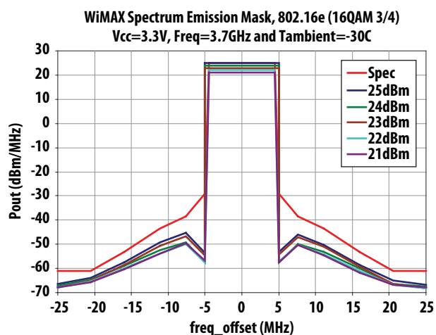
Figure 36. SEM at Vcc=3.3V, -30C and 3.7GHz over Vcc (2dB Post-PA loss assumed)
