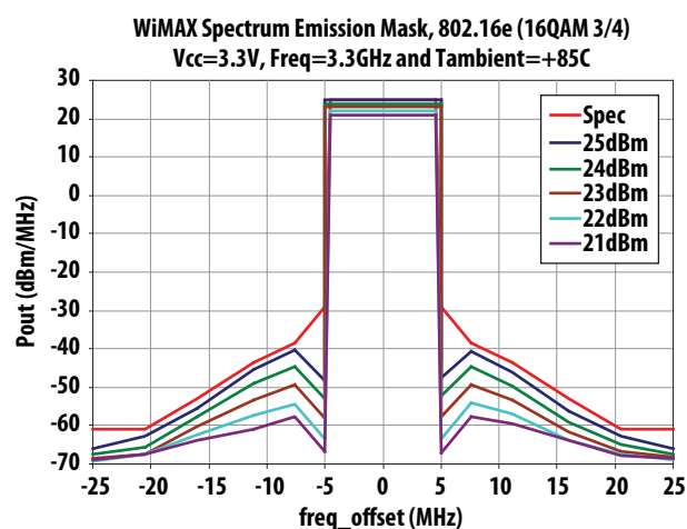
Figure 38. SEM at Vcc=3.3V, +85C and 3.3GHz over Vcc (2dB Post-PA loss assumed)
