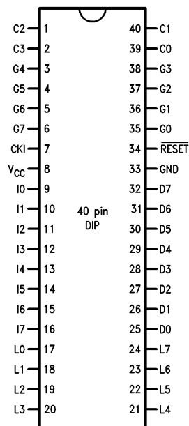
Dual-In-Line Package
