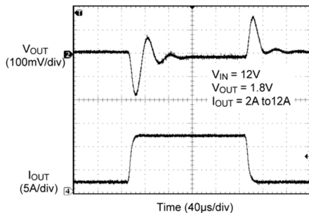
Transient Response
