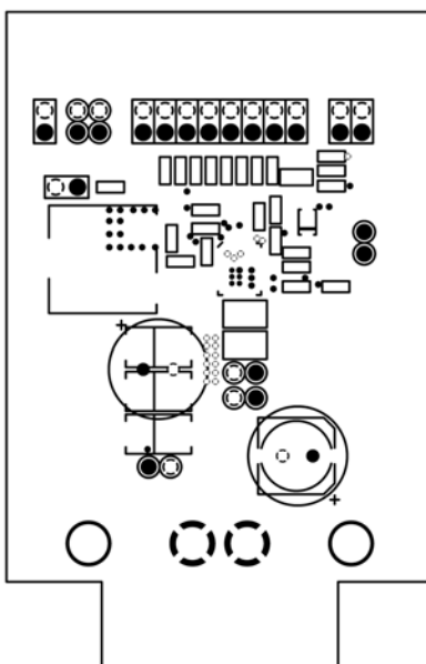
Figure 11. MIC261203 Evaluation Board Mid-Layer 1 (Ground Plane)
