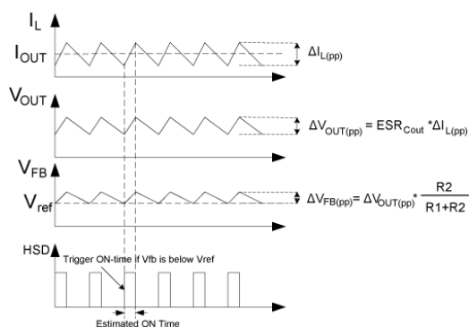
Figure 2. MIC261203 Control Loop Timing
