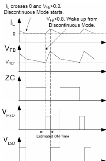
Figure 4. MIC261203 Control Loop Timing (Discontinuous Mode)
