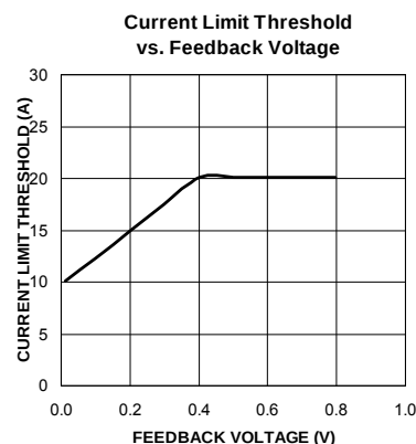
Figure 5. MIC261203 Current-Limit Foldback Characteristic
