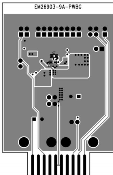
Figure 13. MIC261203 Evaluation Board Bottom Layer
