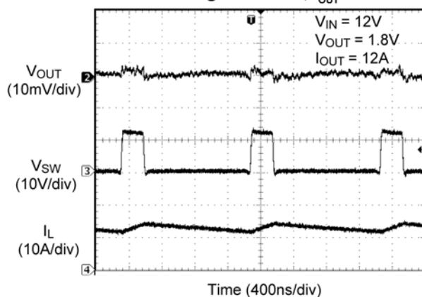
Switching Waveform; I_{OUT} = 12A
