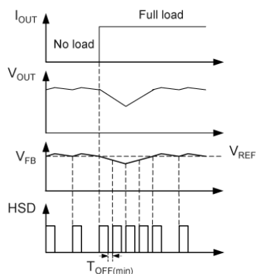
Figure 3. MIC261203 Load Transient Response
