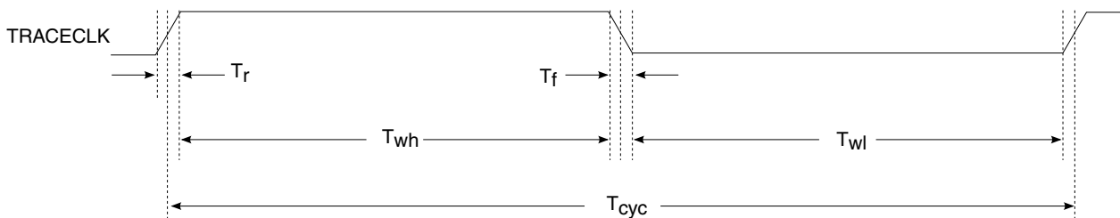
Figure 5. TRACE_CLKOUT specifications
