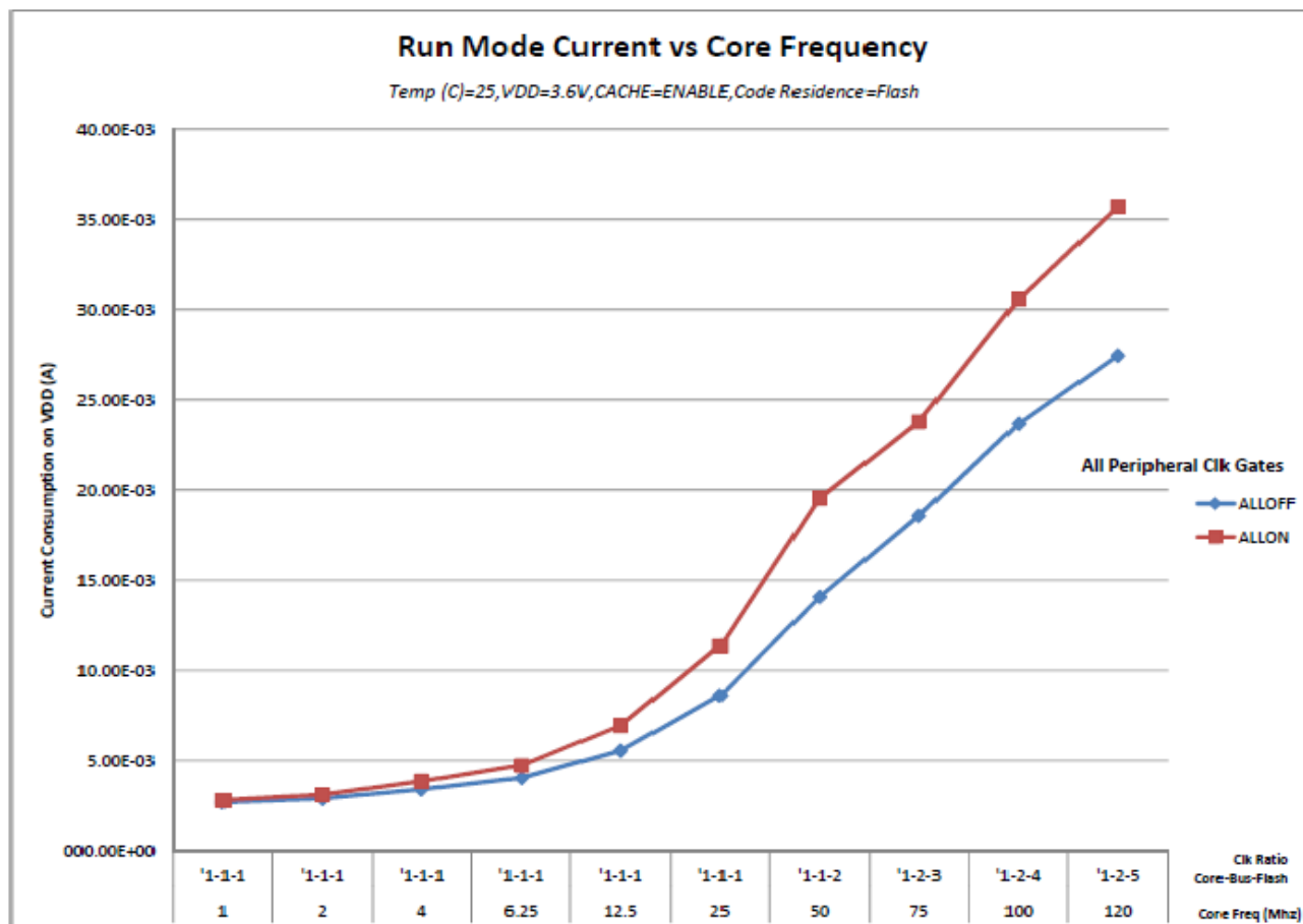
Figure 3. Run mode supply current vs. core frequency
