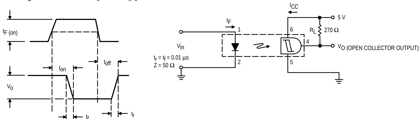
Figure 1. Switching Test Circuit
