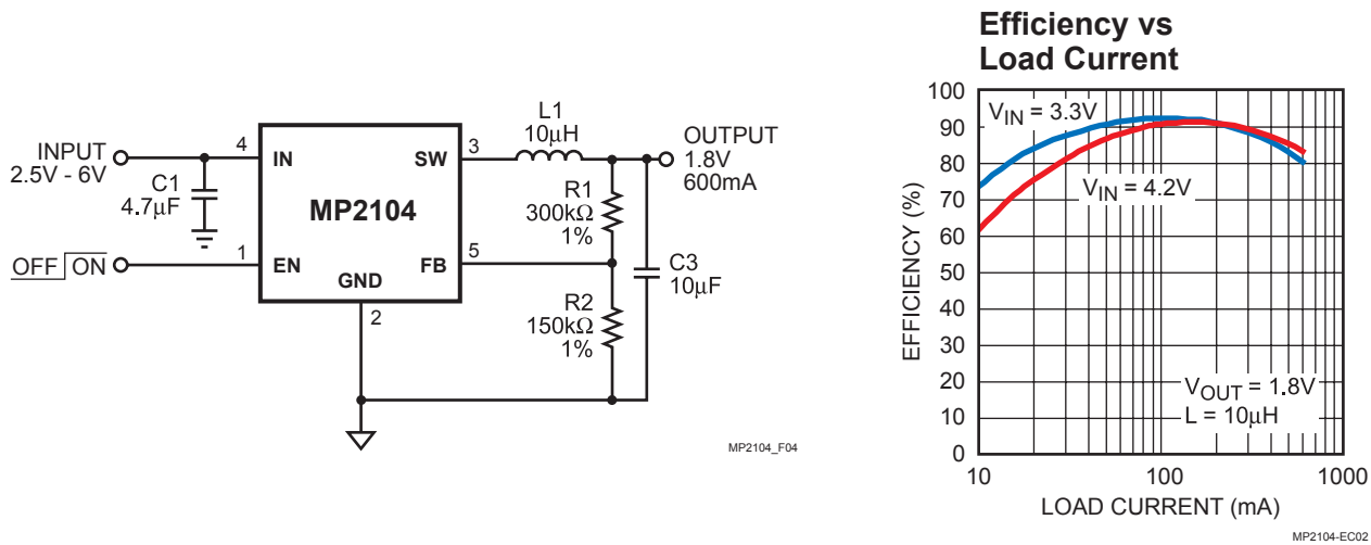
Figure 5— V_{IN} = 2.5V to 6V , V_{OUT} = 1.8V , I_{LOAD} = 600mA Step-Down Circuit ( L = 10\mu H for Higher Light-Load Efficiency)
