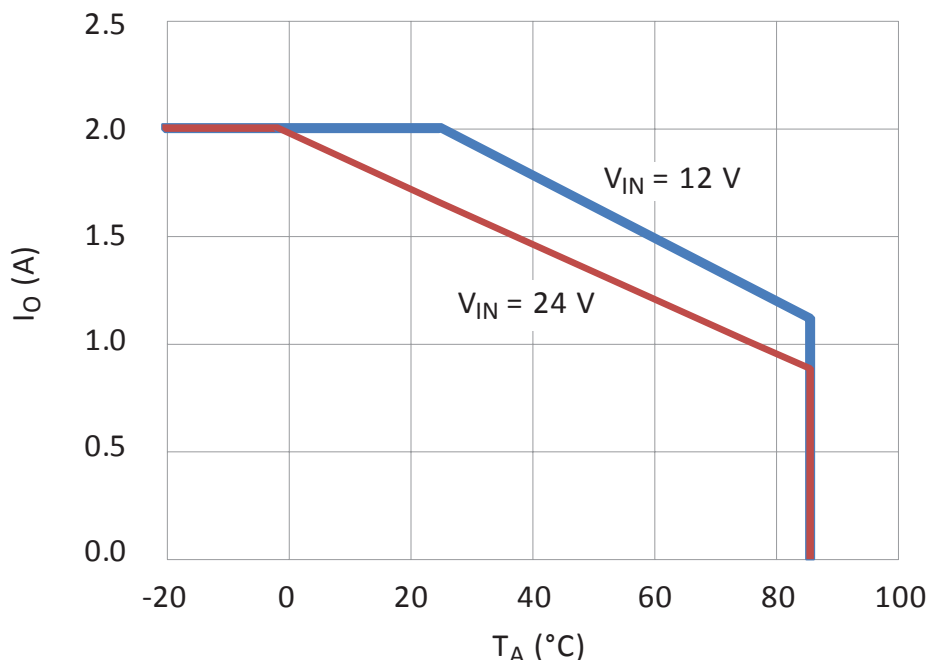
Figure 2. MPM80 thermal derating curve; measurement conditions: V_{\text{O}} = 5\text{ V} , no heatsink
