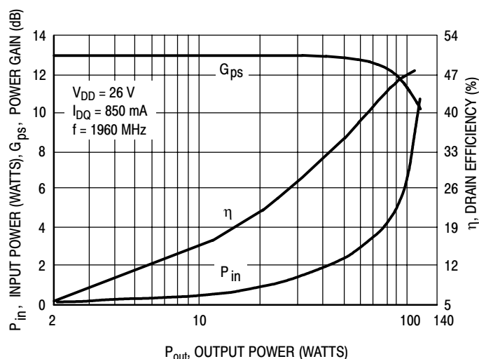
Figure 8. CW Performance
