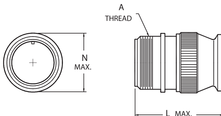
MS3101R Grommet nut, environmental, with grommet®
