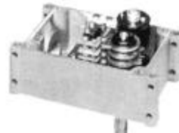
Figure 8 NEMA 1 Enclosure 4 circuit with Gear Coupled Potentiometer
