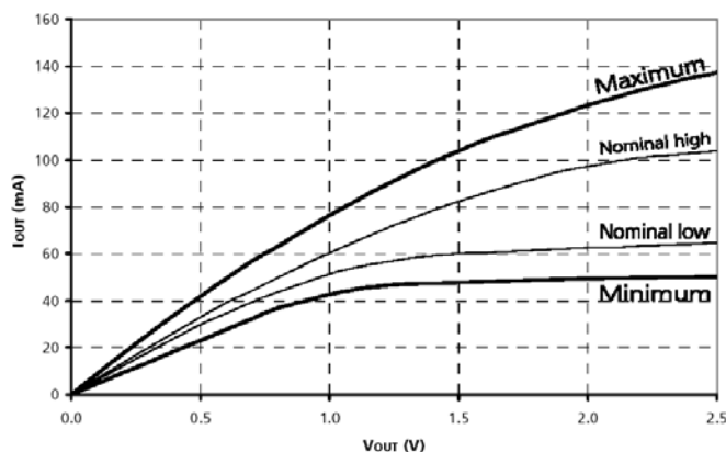
Figure 9: Pull-Down Characteristics
