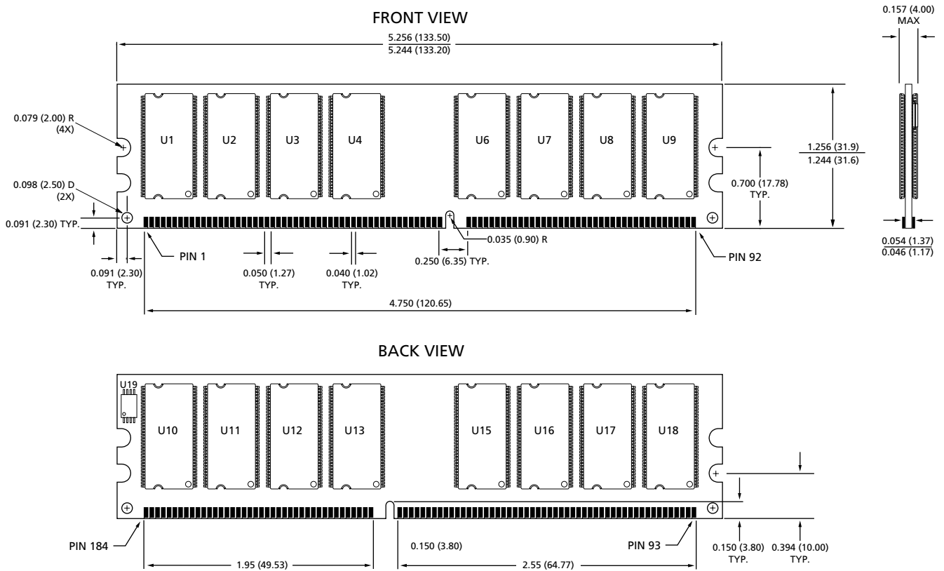
Figure 17: 184-PIN DDR DIMM Dimensions – Standard PCB
