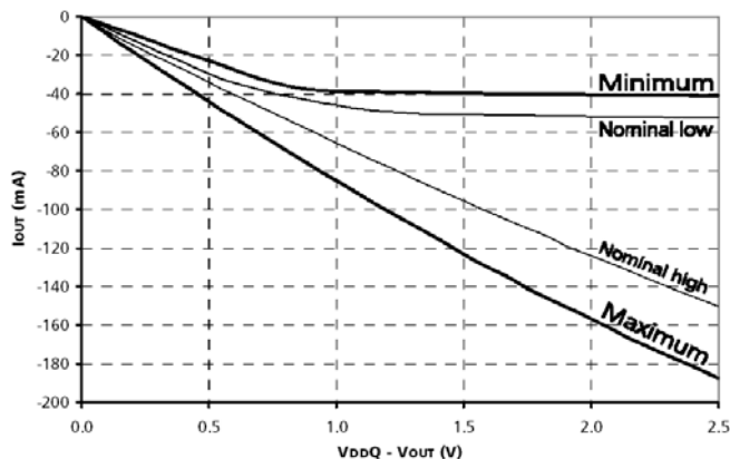
Figure 10: Pull-Up Characteristics
