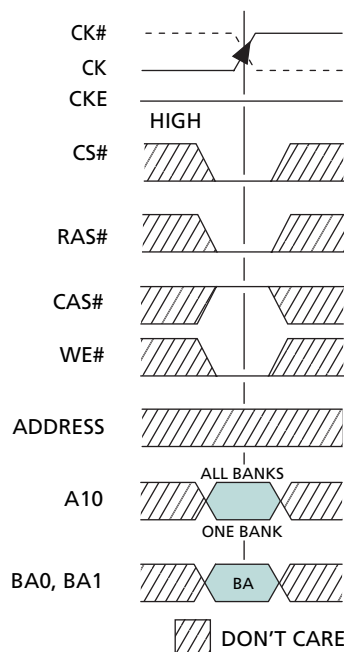
Figure 42: PRECHARGE Command
