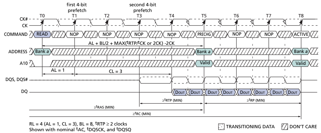
Figure 23: READ-To-PRECHARGE, BL = 8
