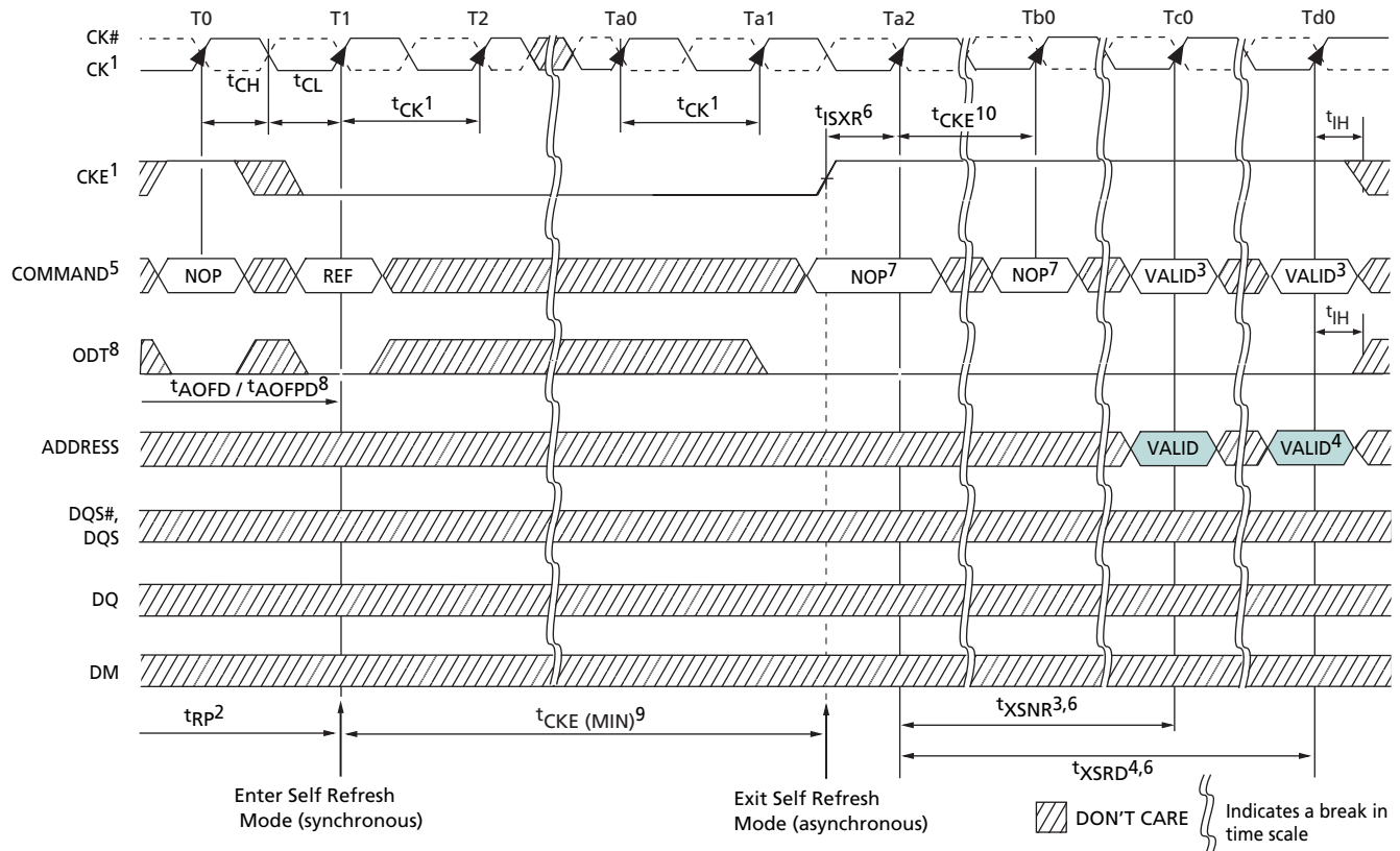
Figure 43: Self Refresh
