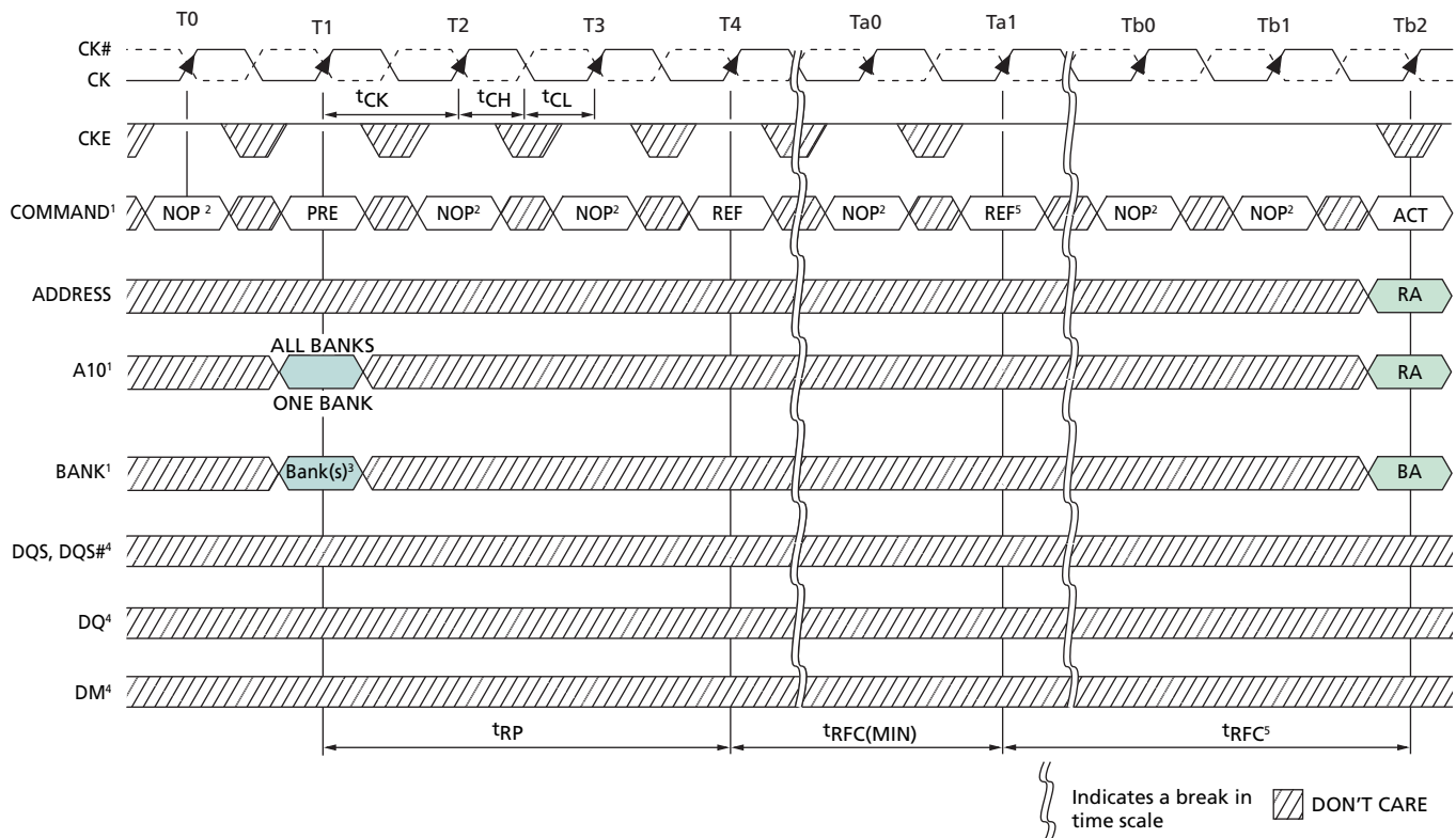
Figure 44: Refresh Mode
