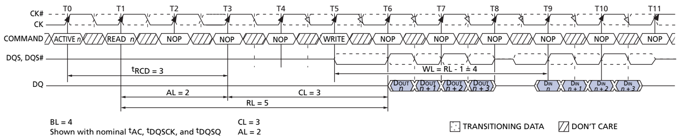
Figure 24: READ-To-WRITE
