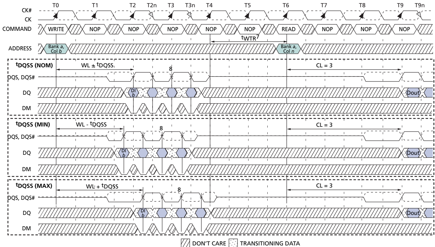
Figure 36: WRITE-To-READ
