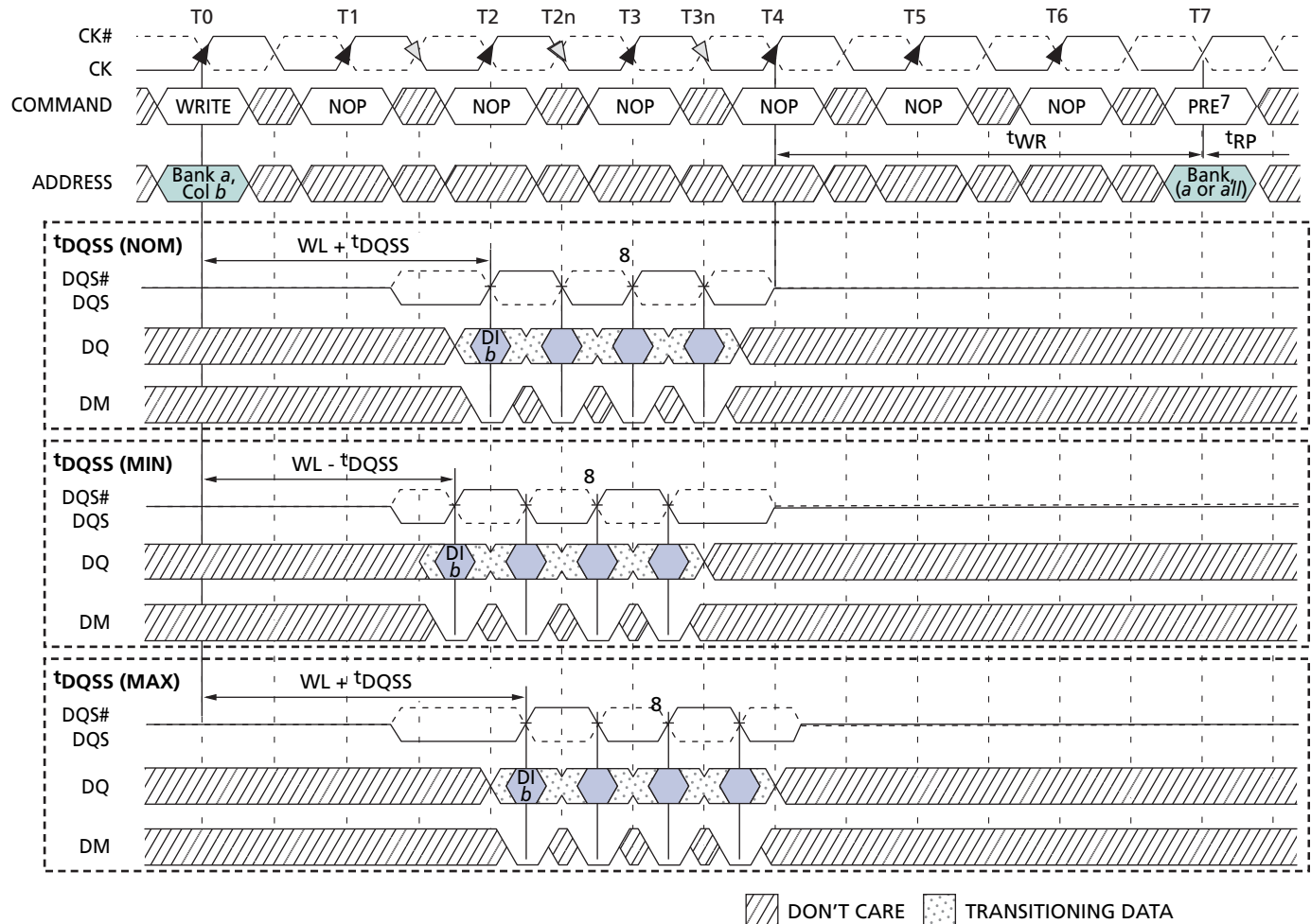
Figure 37: WRITE-To-PRECHARGE
