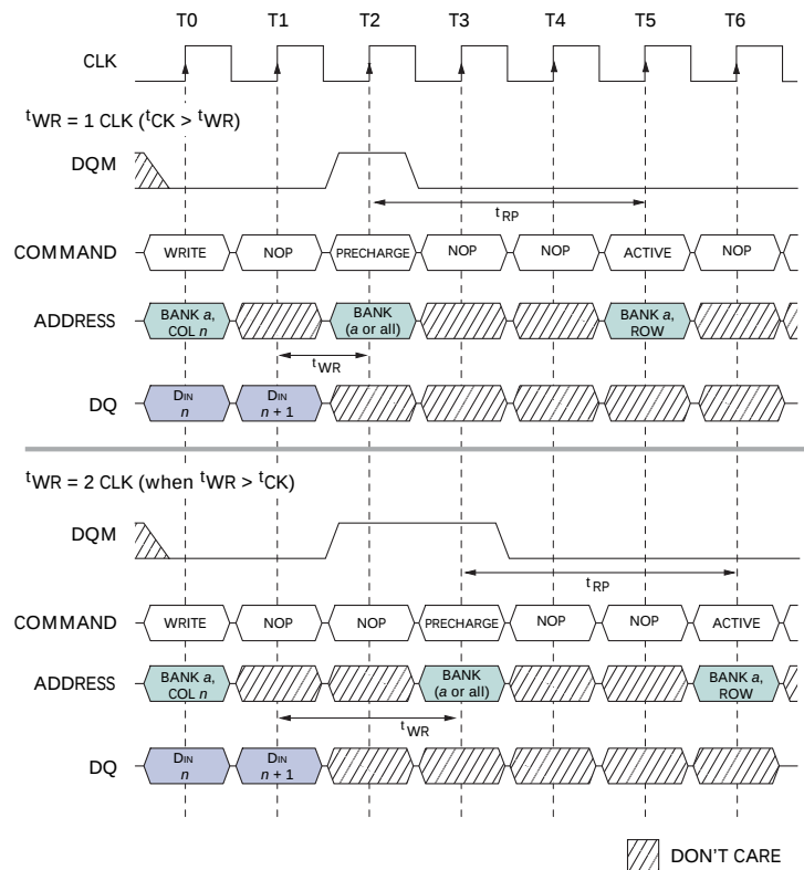
Figure 21: WRITE-to-PRECHARGE
