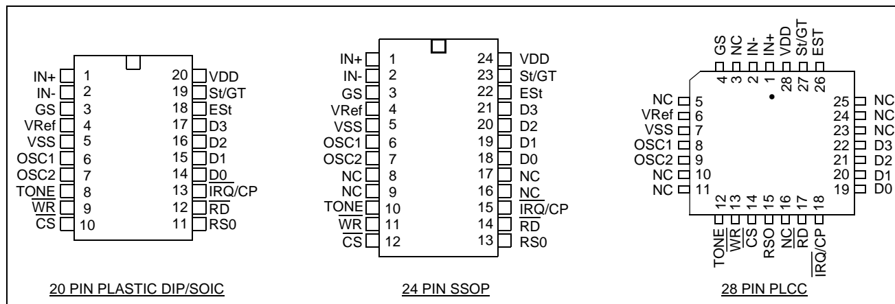
Figure 2 - Pin Connections
