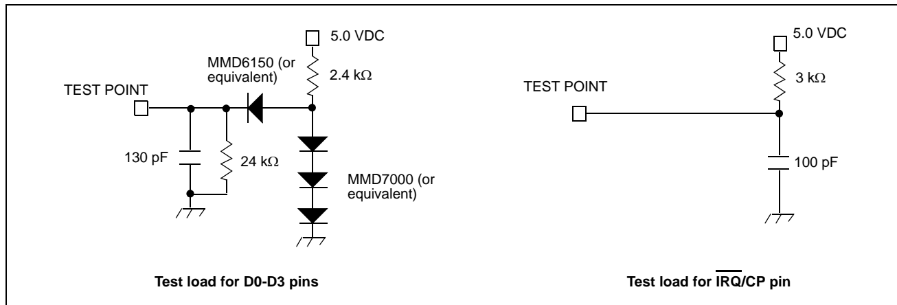
Figure 16 - Test Circuits
